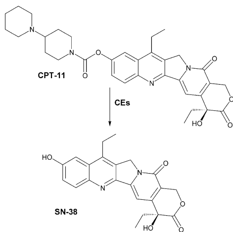
Figure 1. Structure and hydrolysis of CPT-11 by carboxylesterases.
