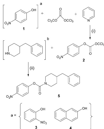
Scheme 1. Synthetic scheme for carbamates. This specific synthesis pictured used p -NP and 4-benzyl piperidine as starting materials. All other carbamate-linked derivatives were prepared using this same general scheme. Starting material (a) used included p -nitrophenol 1 , o -nitrophenol 3 , and \beta -naphthol 4 . The variety of secondary amines (b) used for coupling included 4-benzyl piperidine, 1-benzyl piperazine, 1-(4-chlorobenzylhydrazyl) piperazine, and 1-(2-furosyl) piperazine. Reagents: (i) dichloromethane, 1 h, Ar (ii) pyridine, 12 h, Ar.
